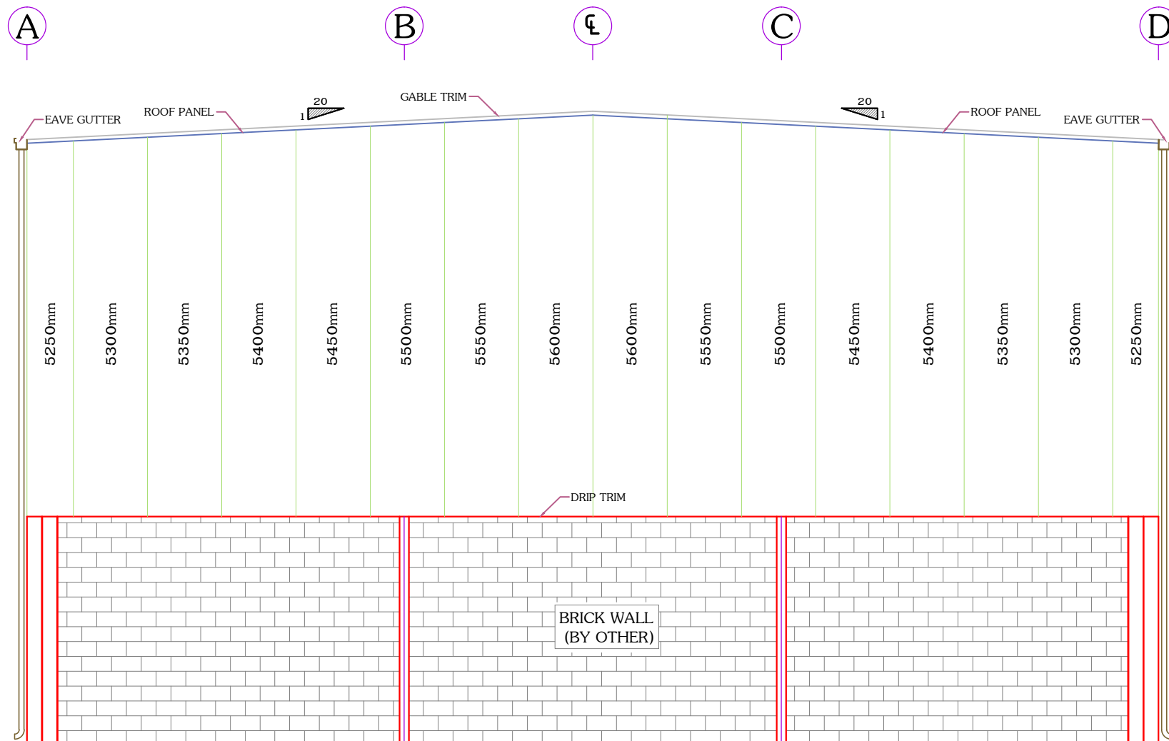
END WALL SHEETING @ GRID-1
